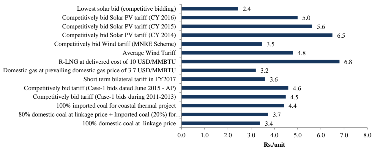
Comparison of cost of generation based on varying fuel mix
